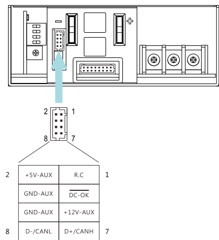
Connect Pin No. Assignment: HRS DF11-8DP-2DS or equivalent
