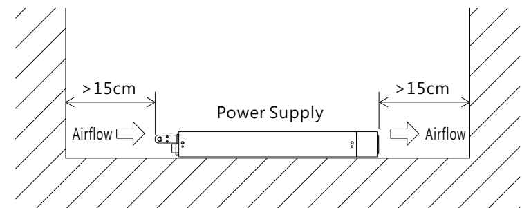
Figure 3-1 Mounting Diagram
