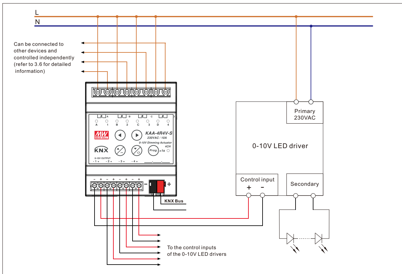
Configuration 2: Work with DC 0-10V LED driver
