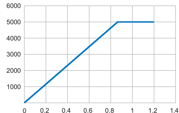
Derating curve VA by operating U
